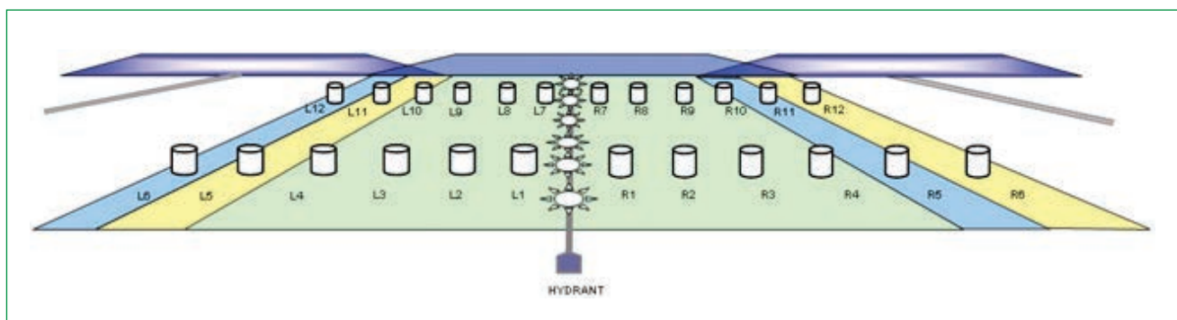
Figure 2.2. Sprayline wetted strip, overlap and collector placement
