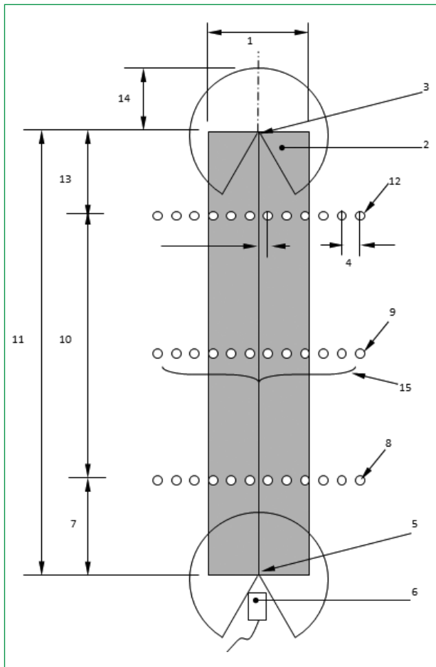
Figure 3.1. Field collector layout (from ISO 8224-1:2002)
