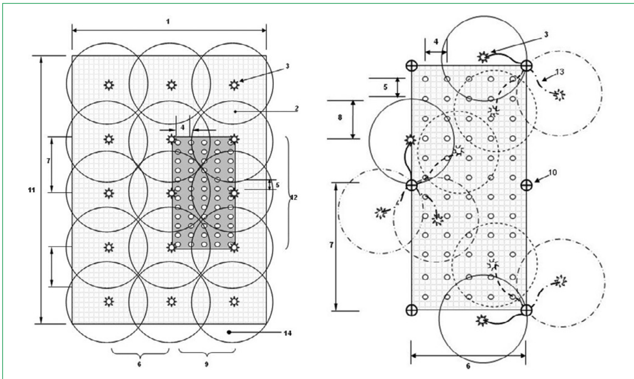
Figure 3.1. Location of sampling grid with a solid-set irrigation area and with a long-lateral system
