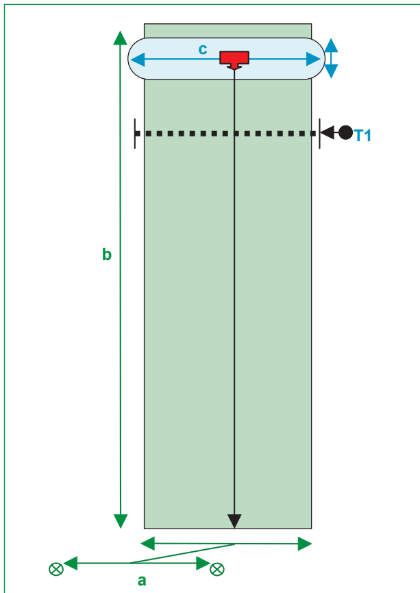
Figure 2.1. Layout of calibration test for travelling irrigators.
