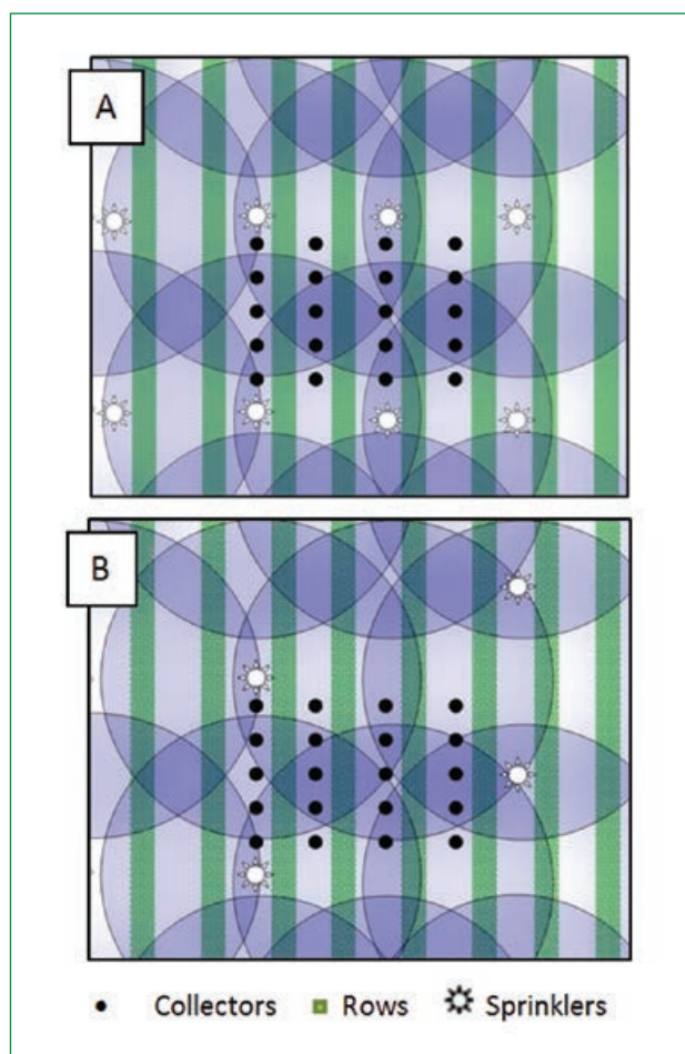
Figure 2.1. Example collector bucket positions relative to rows and sprinklers.
