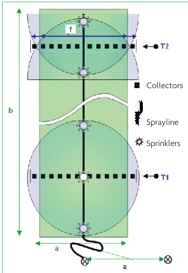
Figure 2.1. Sprayline calibration layout
