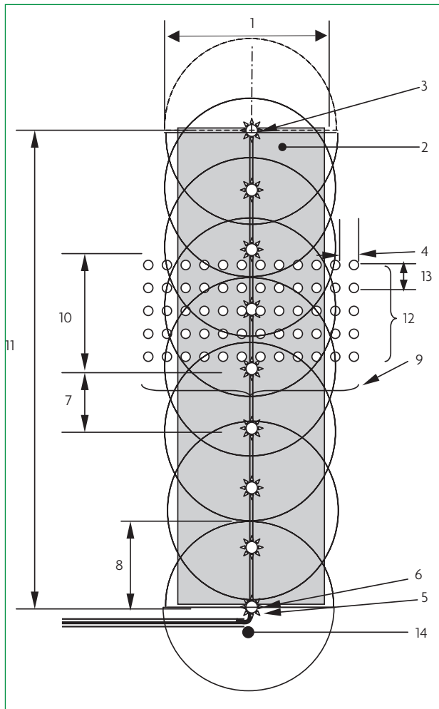
Figure 3.1. Field collector layout for sprayline systems
