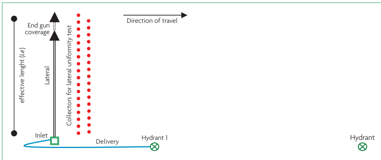
Figure 3.1. Layout of test site for linear move application testing
