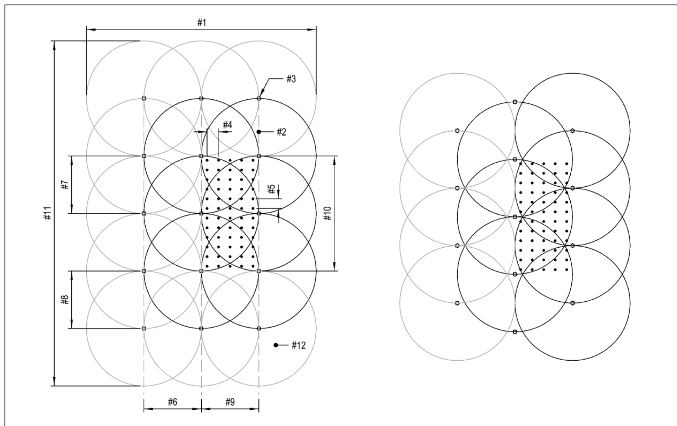
Figure 3.1. Location of sampling grid within a grid sprinkler pattern and a triangular solid-set pattern.
