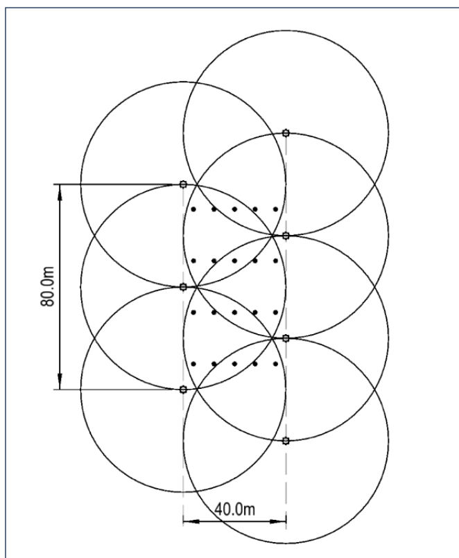
Figure 2.1(B). Example collector bucket positions relative to rows and sprinklers.
