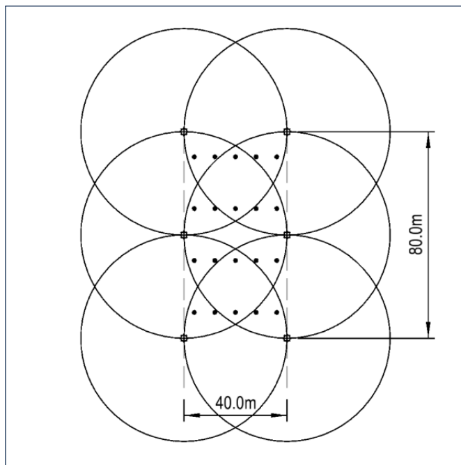
Figure 2.1(A). Example collector bucket positions relative to rows and sprinklers.
