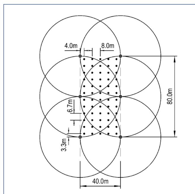
Figure 3.3. The four sprinklers on the right need to operate to ensure the overlap Is measured.
